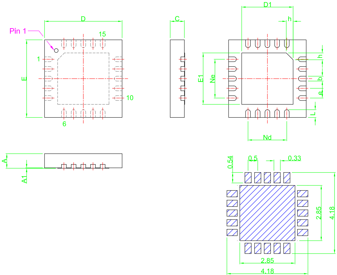
Recommended Land Pattern
