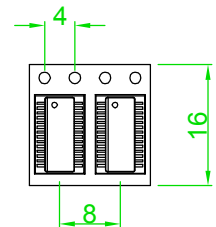
Refer to JEDEC NO. MO-137 AF
