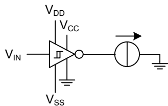
Figure 4. I_{0(SC)}
