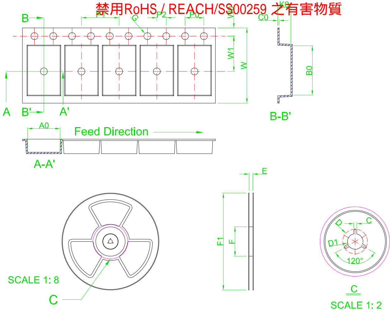
TO-252 T/R
