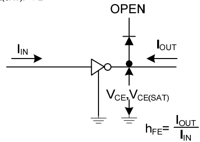
2. V_{CE(SAT)}, h_{FE}
