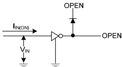
3. I_{IN(ON)}
