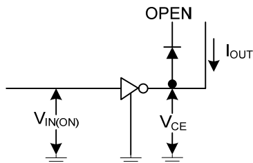
5. V_{IN(ON)}
