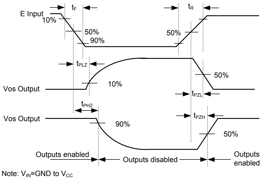
Waveforms showing the turn-on and turn-off times.
