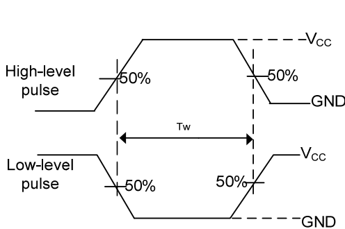
PULSE WIDTH
