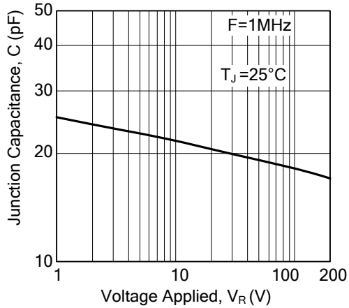
Junction Capacitance Versus Reverse Voltage Applied (Typical Values, Per Diode)
