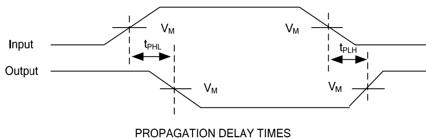
Fig. 2 Propagation delay from input(A) to output(Y) and Output transition time.
